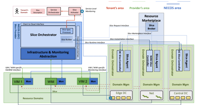
Fig. 1. Abstract view of the NECOS architecture.
