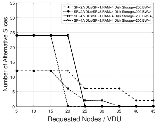
Fig. 7. Number of alternative slices with three resource requirements.
